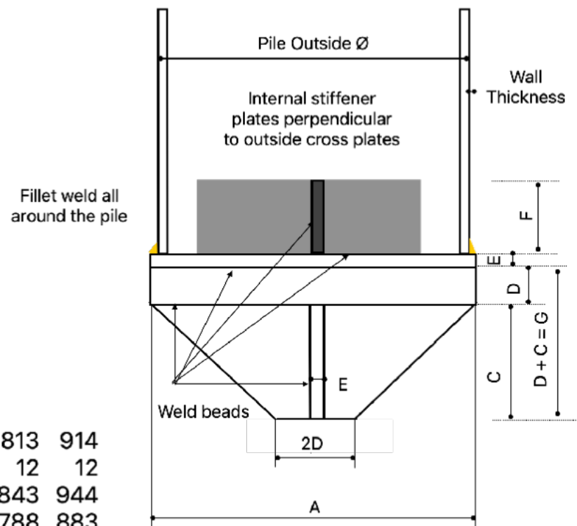
ELEVATION SECTION VIEW
